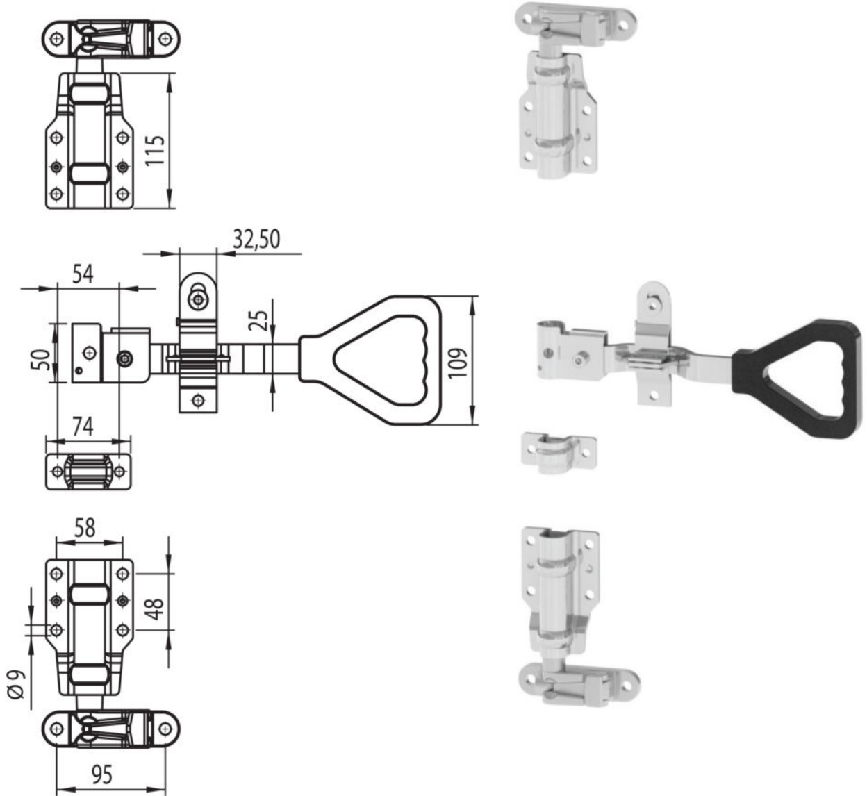
Plastik Kol Set 22 mm Plastic Lever Set 22 mm
